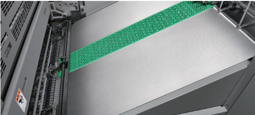
Suction Tape Feeder-type Feeder Board The use of a new feeder board with one belt in the center ensures stable, highly accurate sheet feeding regardless of paper grade or sheet size. Stabilization of sheet surface behavior, sheet travel, and accuracy as well as ease of operation are all improved. Since the Lithrone G40 easily accommodates thick sheets, the time required to prepare for changing the sheet size is shorter.
